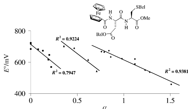
Fig. 1 Influence of the hydrogen bond donor ability \alpha of various families of solvents on the redox potential of Fc-Asp(OBzl)-Cys(Bzl)-OMe (7): (◆) protic solvents (alcohols and acids); (▲) amides and N-bases; (■) others.
