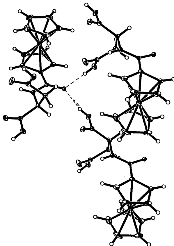
Fig. 3 ORTEP diagram for three adjacent molecules of 8 engaged in H-bonding. Two acid OH are H-bonded with the Fc–C=O group. The water molecule has been omitted for clarity.
