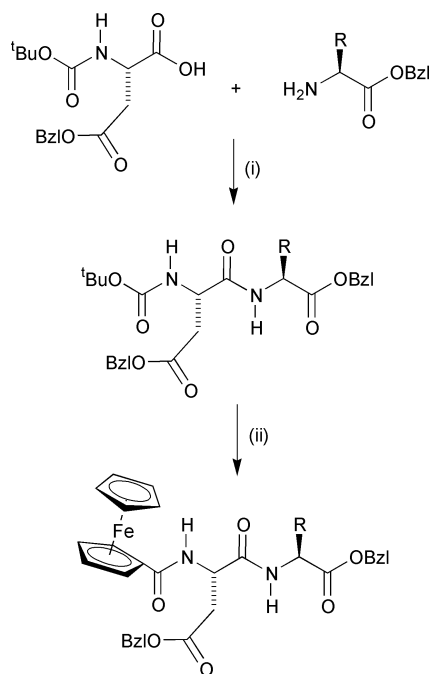
Scheme 1 General scheme for the synthesis of ferrocenyl-dipeptides. (i) EDC, HOBT, Et 3 N, CH 2 Cl 2 , RT; (ii) (a) TFA, CH 2 Cl 2 ; (b) FcCOOH, EDC, HOBT, Et 3 N, CH 2 Cl 2 , RT.
