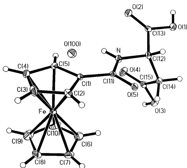
Fig. 2 ORTEP diagram for Fc-Asp(OH)-OH · 1/3H 2 O ( 8 · 1/3H 2 O) showing a single molecule of 8 and the water molecule occupying a position allowing its interaction with CH(5) and the amide NH.
