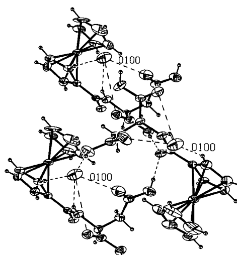
Fig. 4 Stereoscopic view of the extensive H-bonding network present in the solid state between the water molecule (O100) and three adjacent molecules of 8 . In addition to “conventional” O···H–N and O–H···O=C H-bonding, the water molecule is also involved in C–H···O interactions with the Cp ring.
