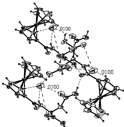
Fig. 4 Stereoscopic view of the extensive H-bonding network present in the solid state between the water molecule (O100) and three adjacent molecules of 8 . In addition to “conventional” O···H–N and O–H···O=C H-bonding, the water molecule is also involved in C–H···O interactions with the Cp ring.
